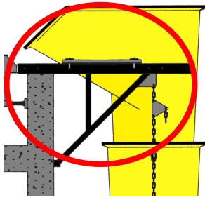
#519 PARAPIT OUTRIGGER TRASH HOPPER BRACKET ONLY $13 DAY | $26 WK
